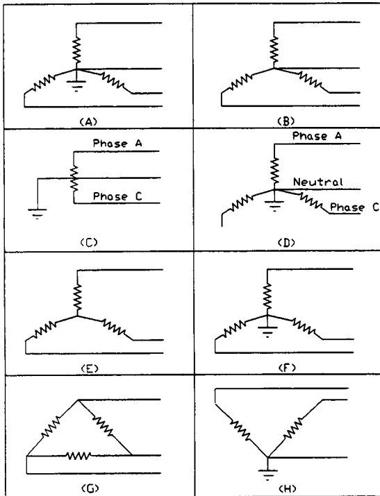
Fig. 6 Acceptable Supply Voltages
