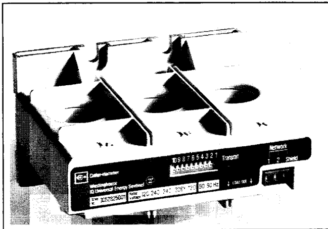
Fig. 1 IQ Universal Energy Sentinel - Internal CT Version
