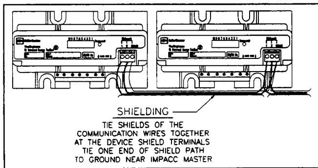
Fig. 4 Network Interwiring
