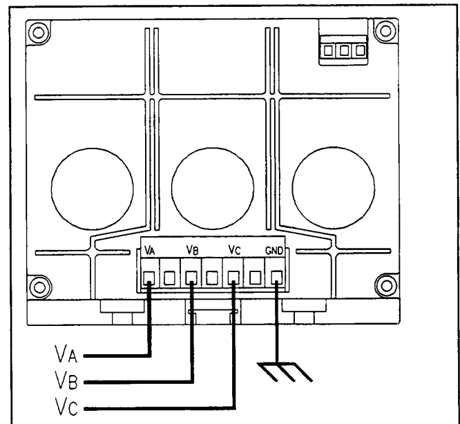
Fig. 3 IQ Universal Energy Sentinel Voltage Connection
