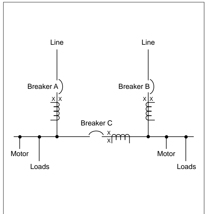
Figure 5-7 Power Distribution
