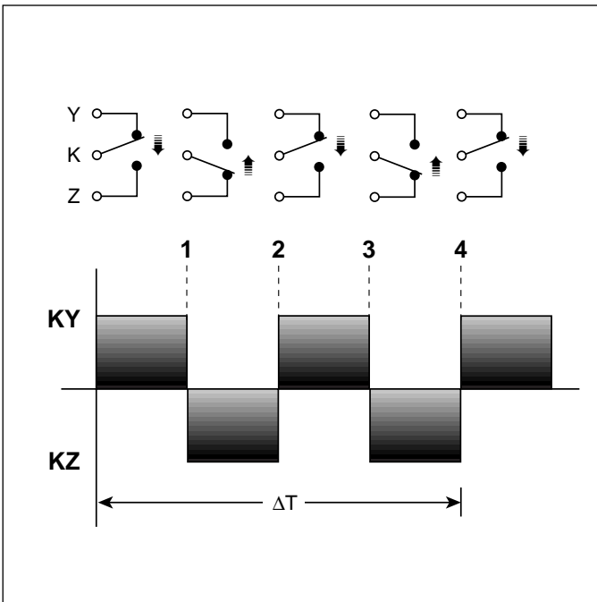
Figure 5-22 3-Wire Pulse Train
