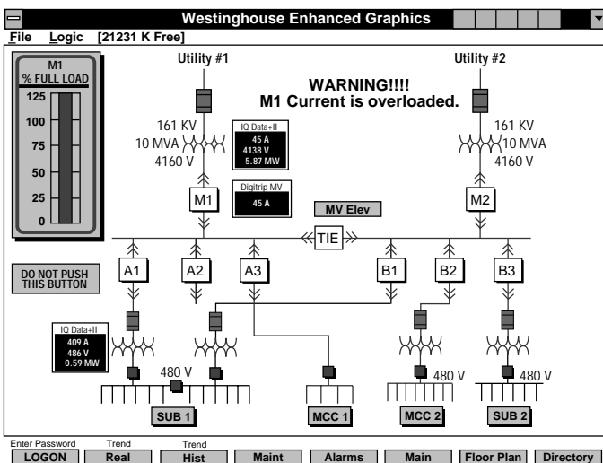
Figure 5-37 Typical Enhanced Graphics Screen
