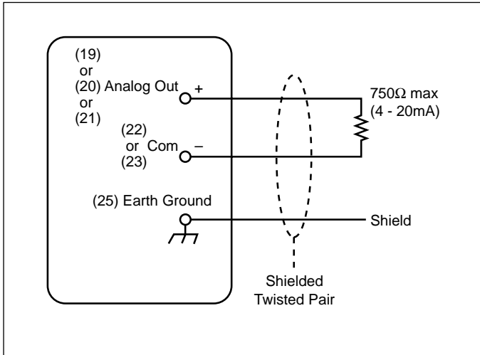
Figure 5-17 Analog Output Connections 4-20 or 0-20mA
