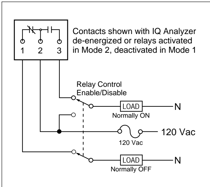
Figure 5-19 Typical Relay Output Connections
