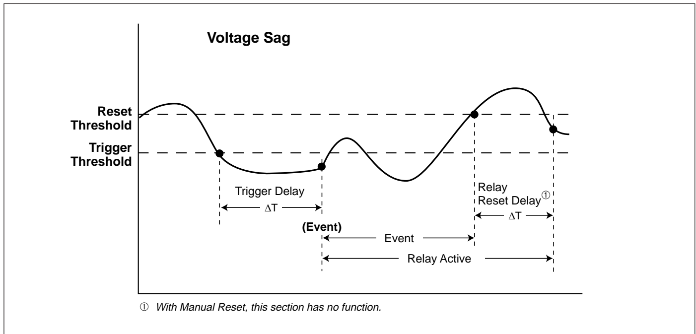
Figure 5-26 Representation of IQ Analyzer's Handling of Setting Driven Alarms
