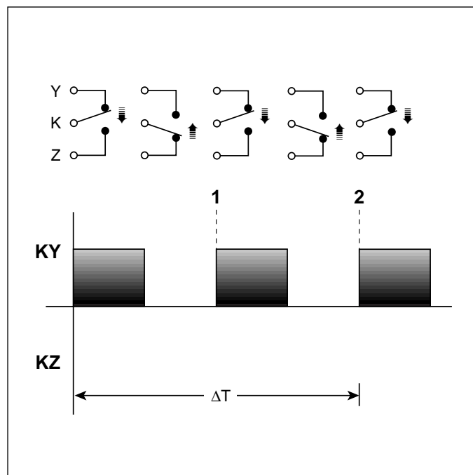
Figure 5-21 2-Wire Pulse Train
