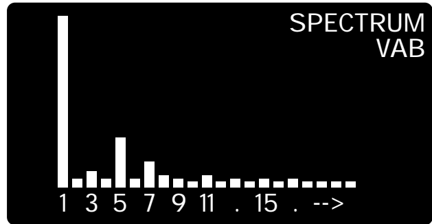
Figure 5-39 Typical Harmonic Spectrum Display
