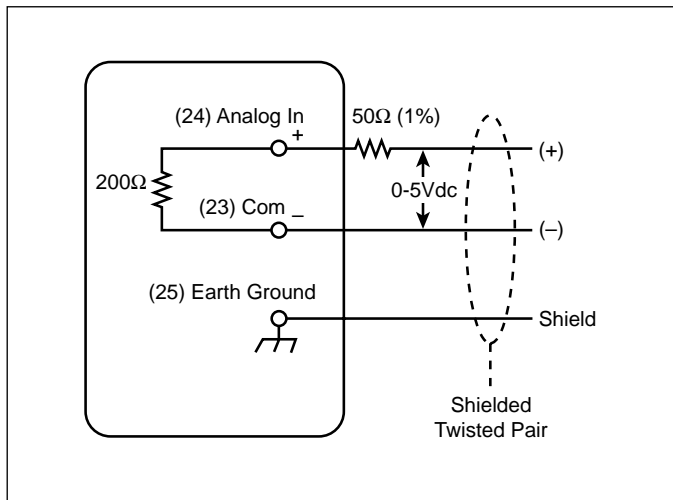
Figure 5-16 Connections for 0-5Vdc Input Signal
