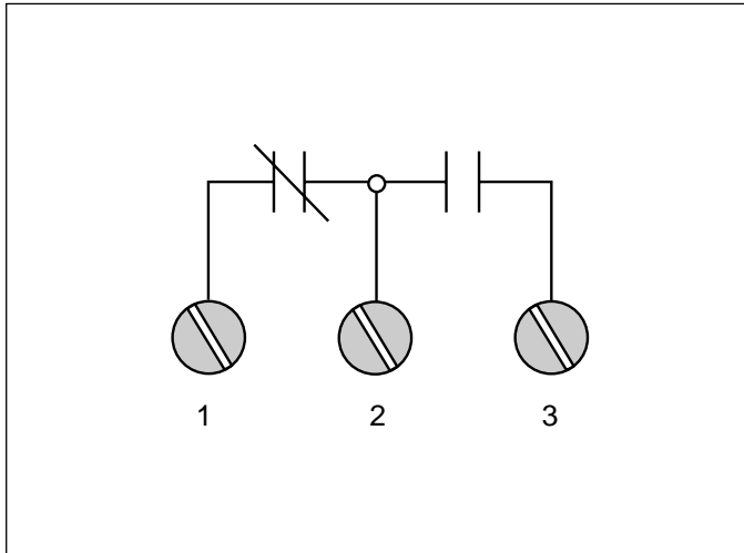
Fig. 5-18 Relay Contact with IQ Analyzer De-energized
