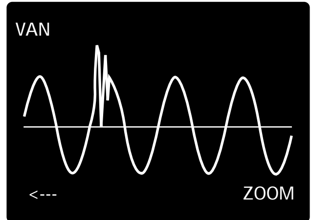
Figure 5-28 Typical Transient Waveform Display on IQA-6200 Series
