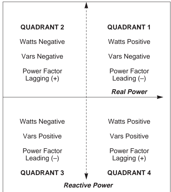
Figure 5-5 Power Quadrants, Power Engineers
