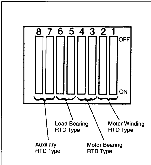
Fig. 3 DIP Switch
