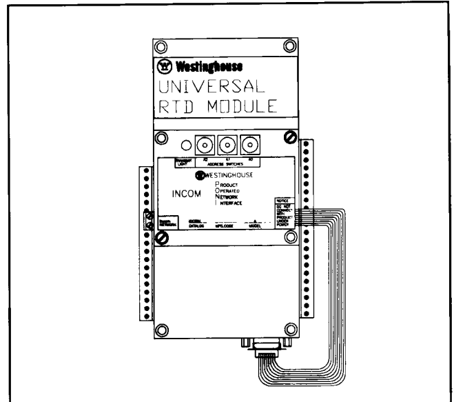
Fig. 8 RTD Module with PONI Card Mounted
