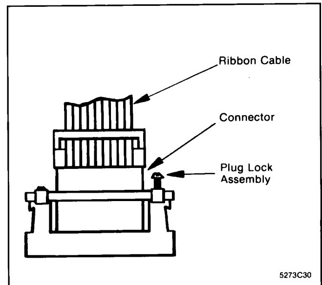
Fig. 9 Plug Lock Assembly
