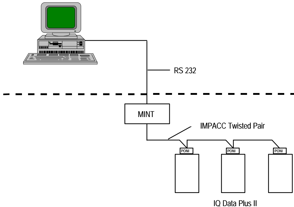
Personal Computer with Factory Link and EDI
