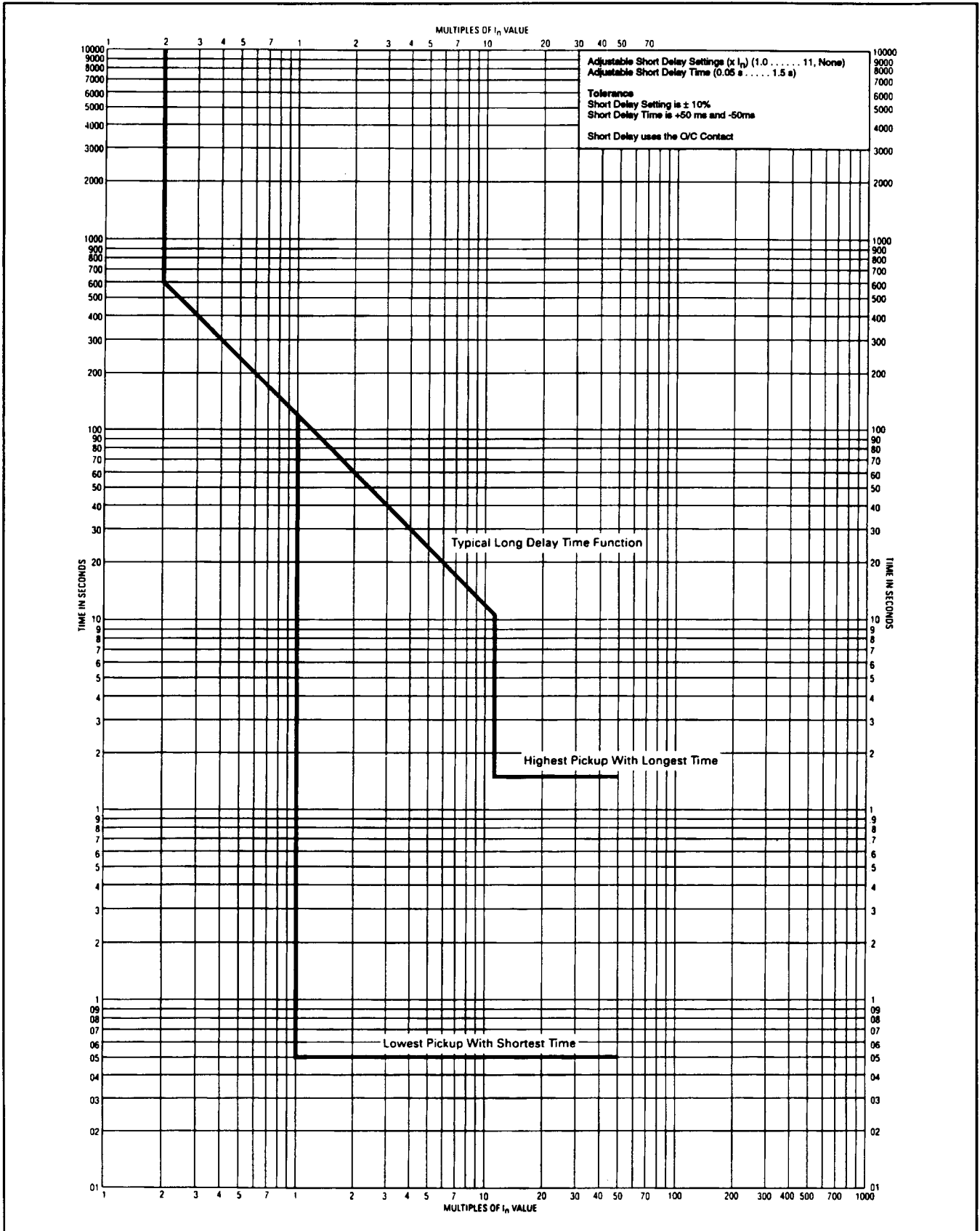
Figure 7-5 Short Delay Phase Curves, (SC-5394-92).
