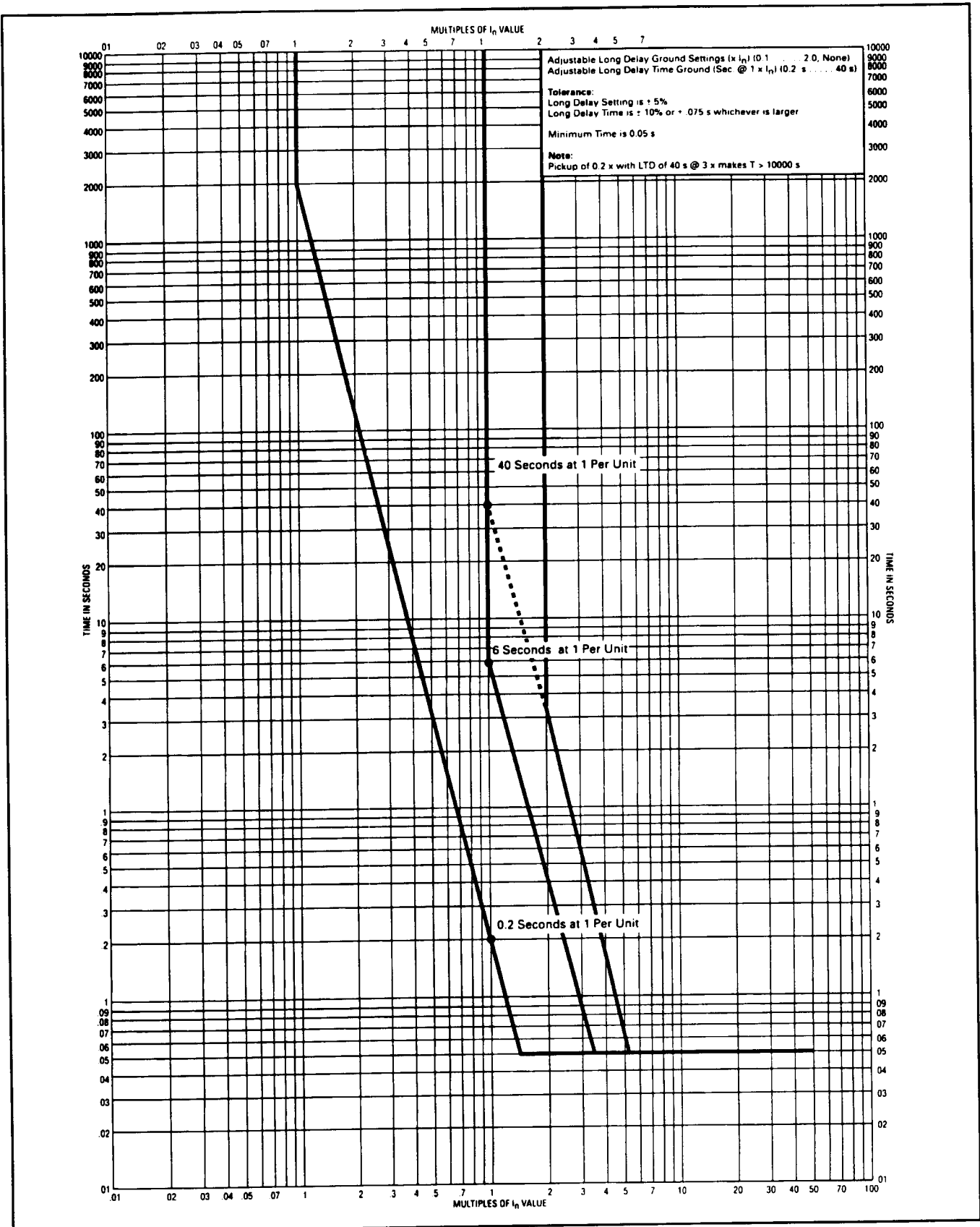
Figure 7-8 Long Delay Ground, I^4T Curves (SC-5399-92).
